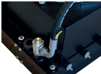
Externer Bypass External Bypass
