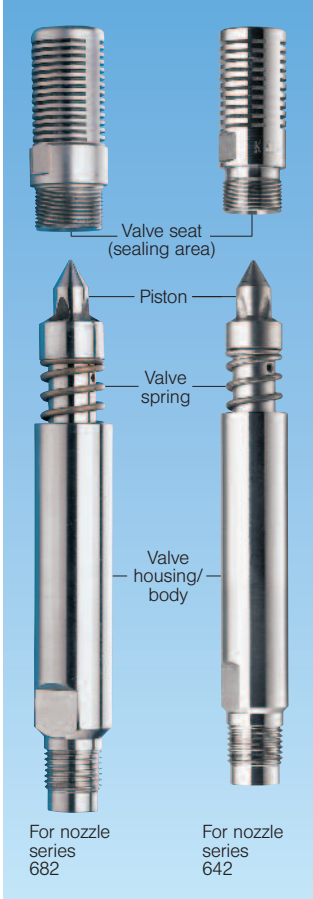
WSV Water Stop Valve, components
