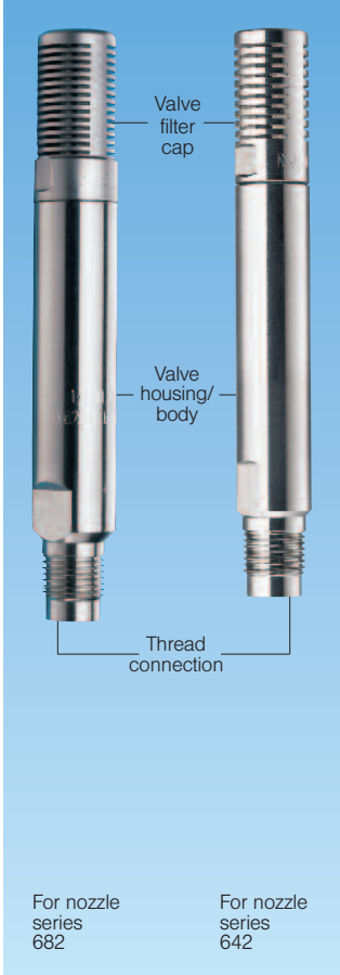
WSV Water Stop Valve
